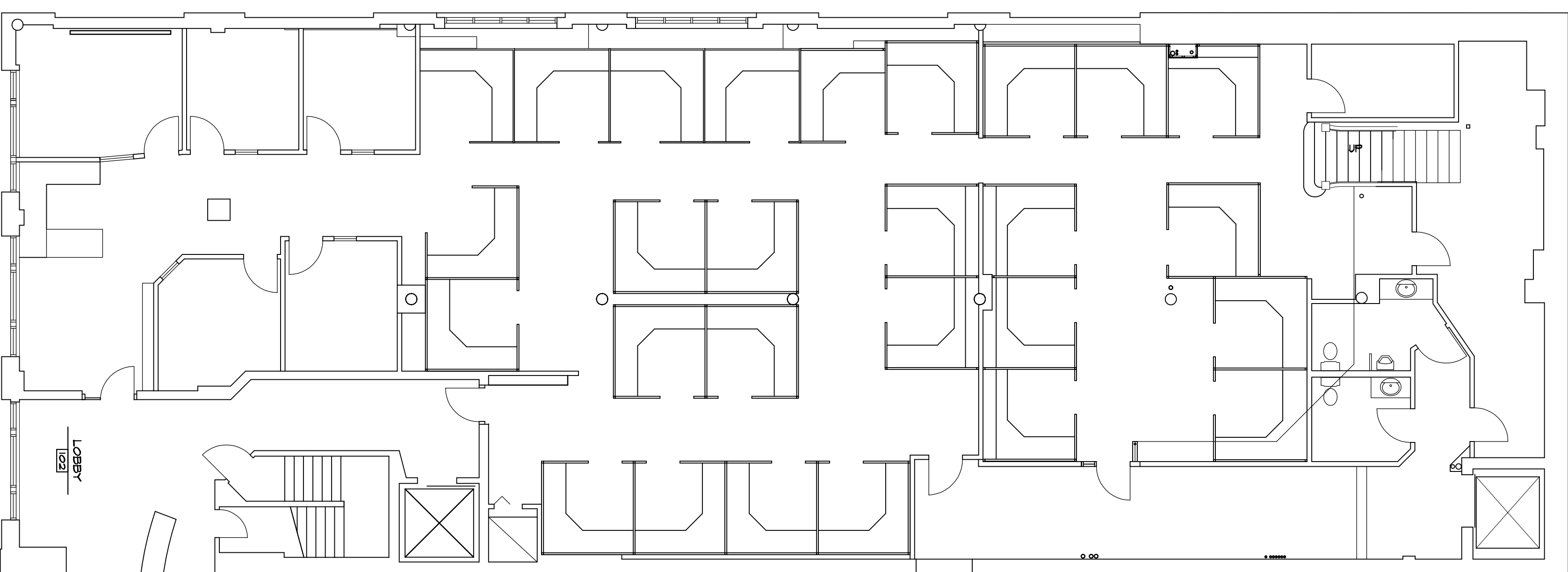
FIRST FLOOR PLAN 1/8" = 1'-0"
