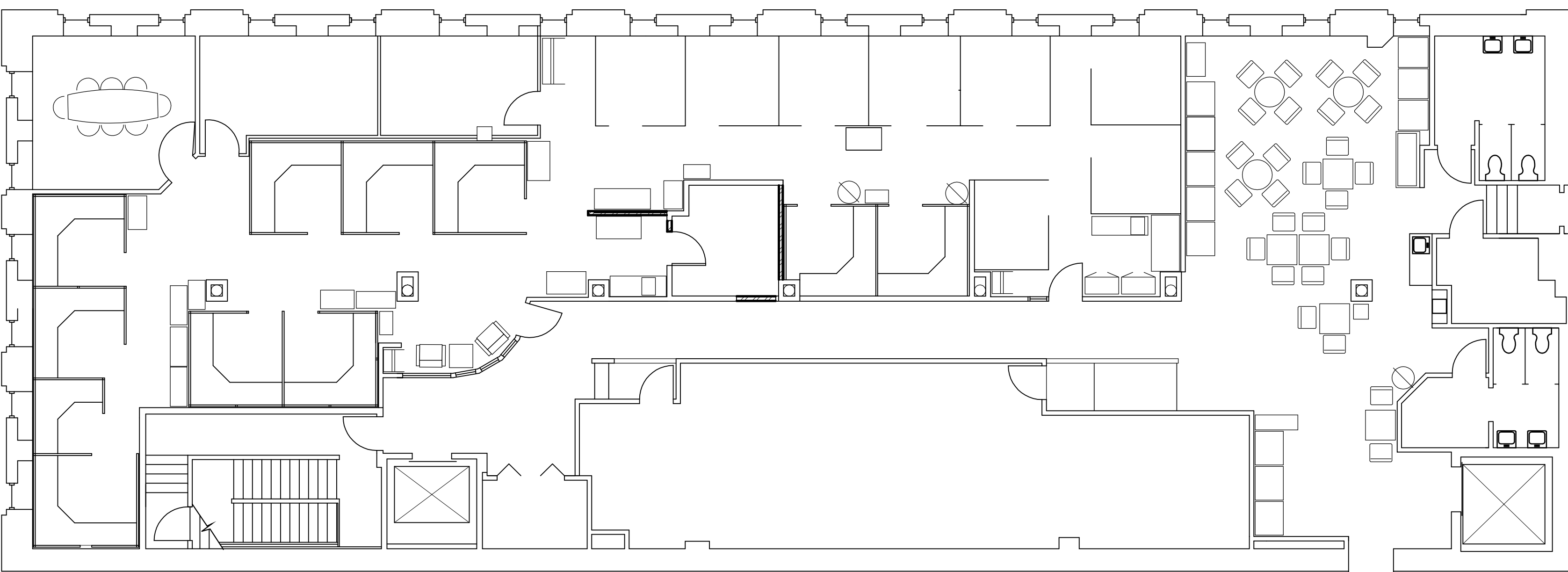
THIRD FLOOR PLAN 1/8" = 1'-0"
